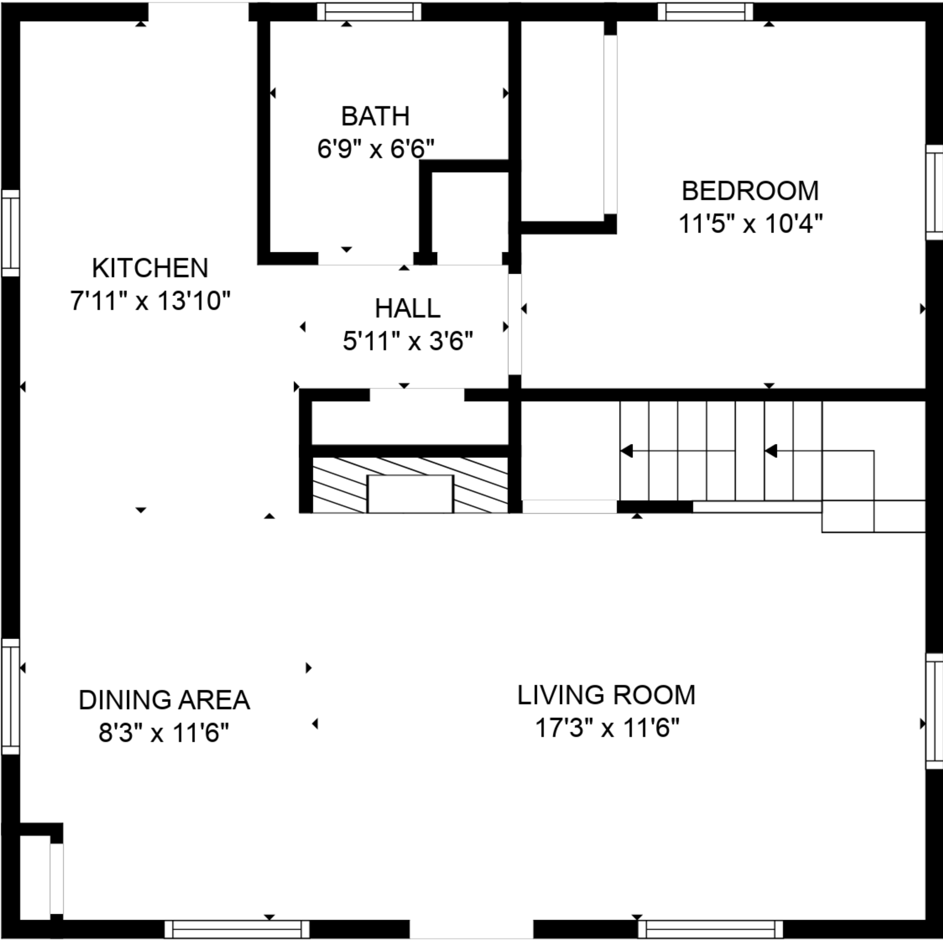
FLOOR 2
